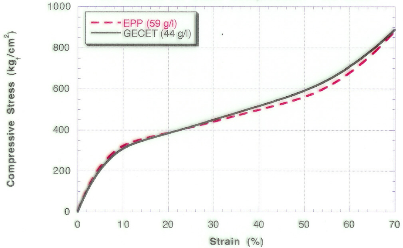
Compressive Stress vs. Strain Test Method for Static Compression - JIS Z0234
